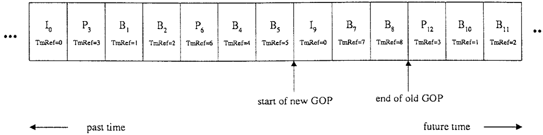
Figures 3A and 3B: Compressed and Displayed Order
